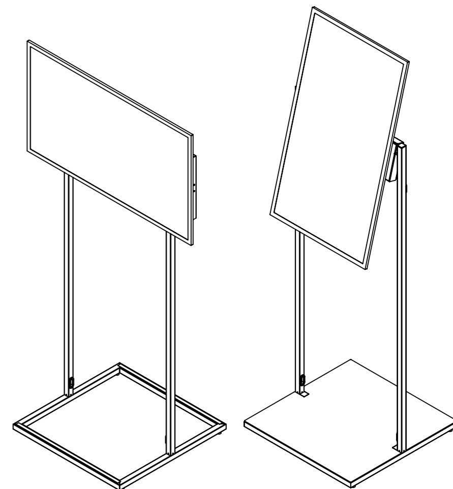
ISOMETRIC VIEW LANDSCAPE WITHOUT BASE COVER ISOMETRIC VIEW PORTRAIT WITH BASE COVER
